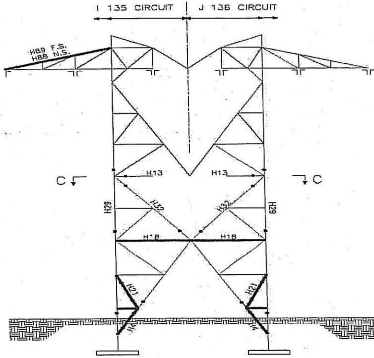
Figure 1: Lattice Tower
