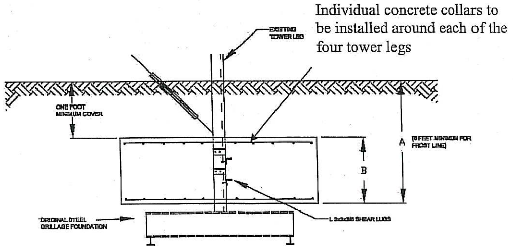
Figure 2: Concrete Collar*
